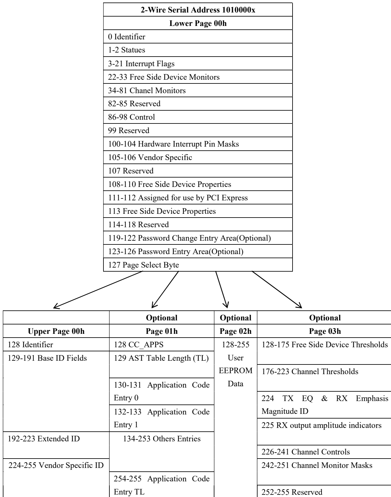
Figure 2 –QSFP28 Memory Map
